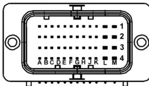
Figura 2: Conector PR-8
